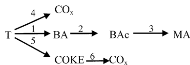
Fig. 6. Reaction network.
