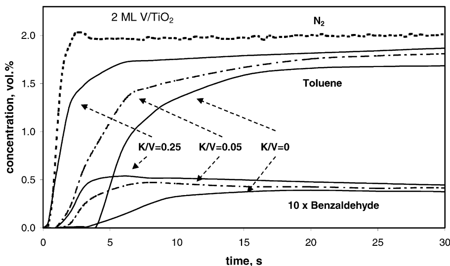
Fig. 4. Transient response curves obtained at 573 K after the switch of the Ar flow to the 2 vol.% toluene/98 vol.% Ar flow over the pre-oxidised catalysts containing 2 ML of vanadia and different K/V ratios (catalyst loading corresponds to 4.0 \text{ m}^2 ).
